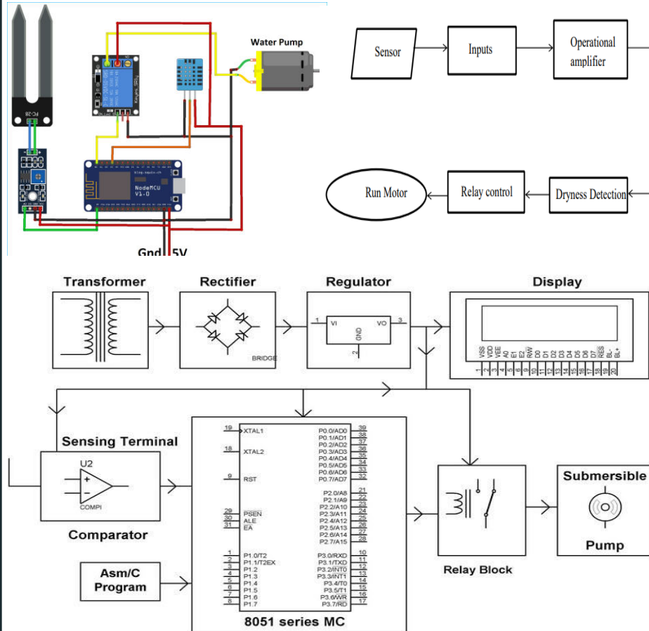
Block Diagram of Soil Moisture Content Based Irrigation
