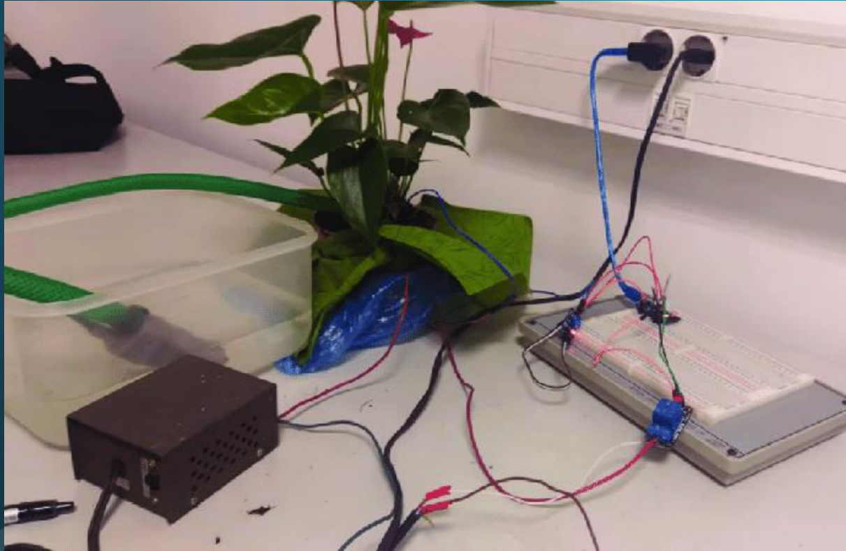
Testing the automatic plant watering system
