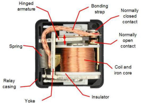
Relay internal structure
